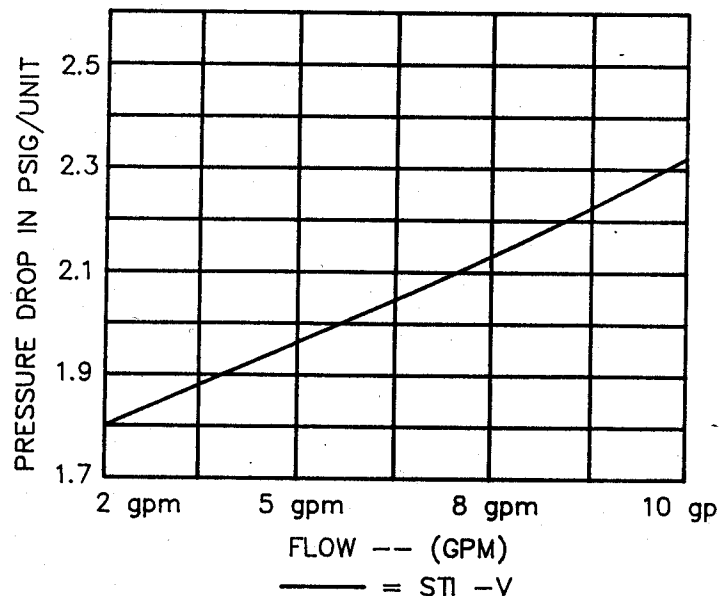
SERVICE TECH 200 HP & IRON .160 HP PRESSURE DROP CURVE
