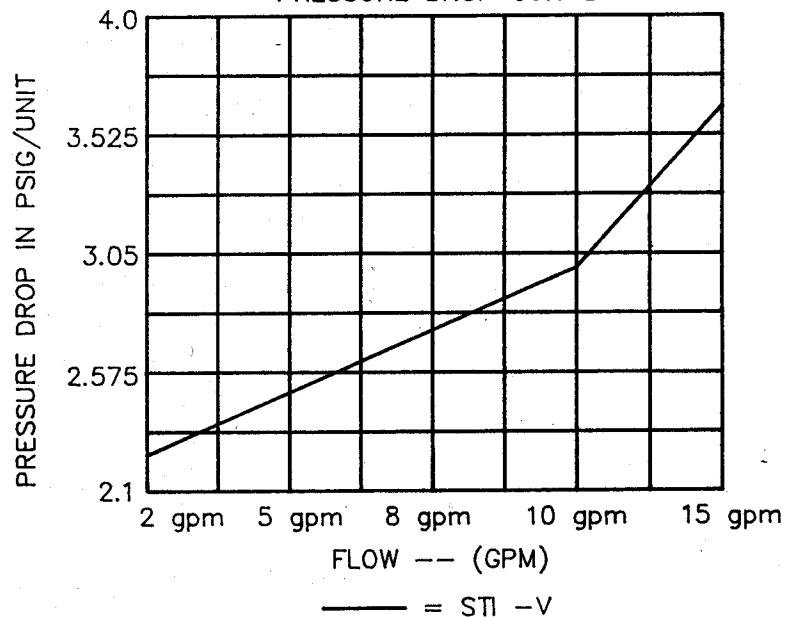
SERVICE TECH 300 HP PRESSURE DROP CURVE
