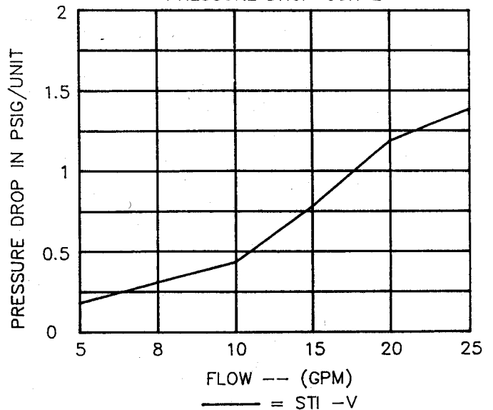
SERVICE TECH 500 HP & IRONMASTER 450 HP PRESSURE DROP CURVE
