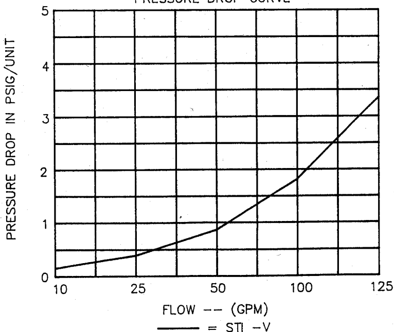
SERVICE TECH 2500 HP PRESSURE DROP CURVE
