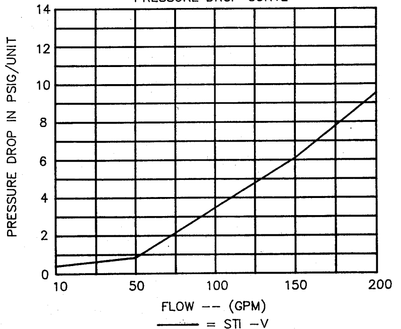
SERVICE TECH 5000 HP PRESSURE DROP CURVE
