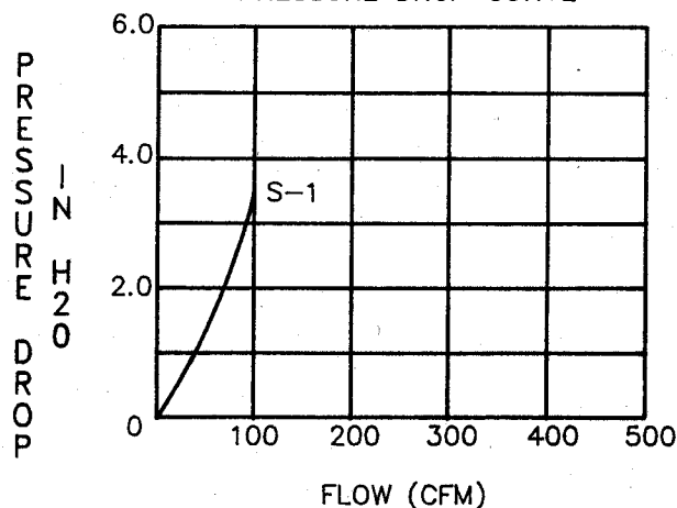
SERVICE TECH S-1 PRESSURE DROP CURVE
