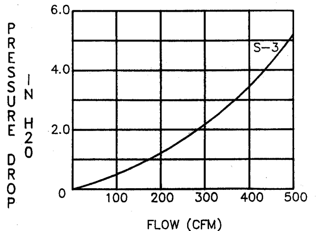
SERVICE TECH S-3 PRESSURE DROP CURVE
