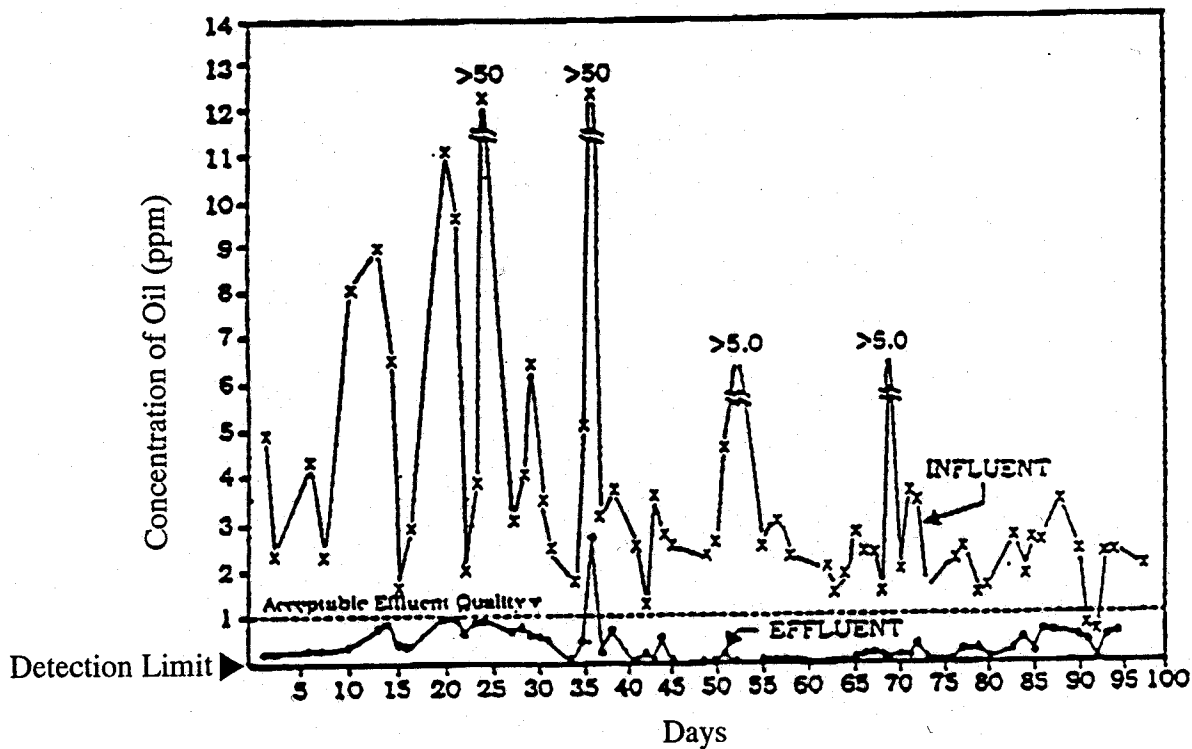
FIGURE 1. Influent and Effluent Oil Concentrations
